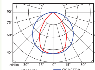
LAURA LED 2M 71°
