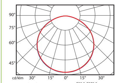
LAURA LED 2M 117°
