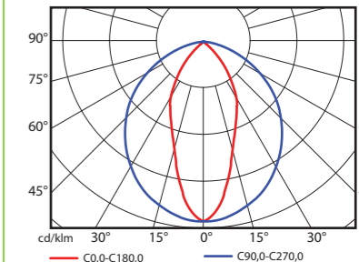
LAURA LED 2M 41°
